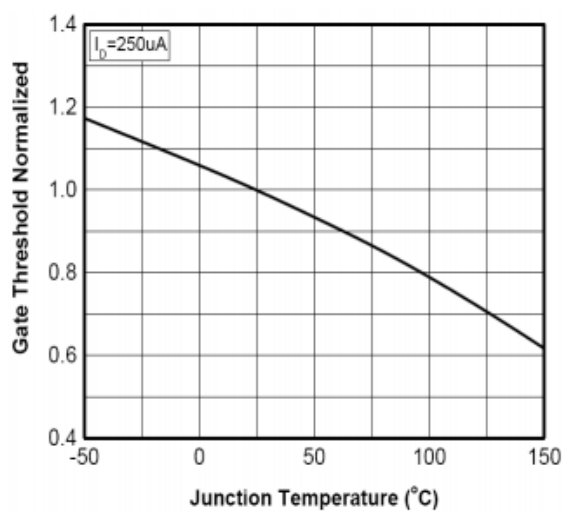
Normalized V_{GS(th)} characteristics
