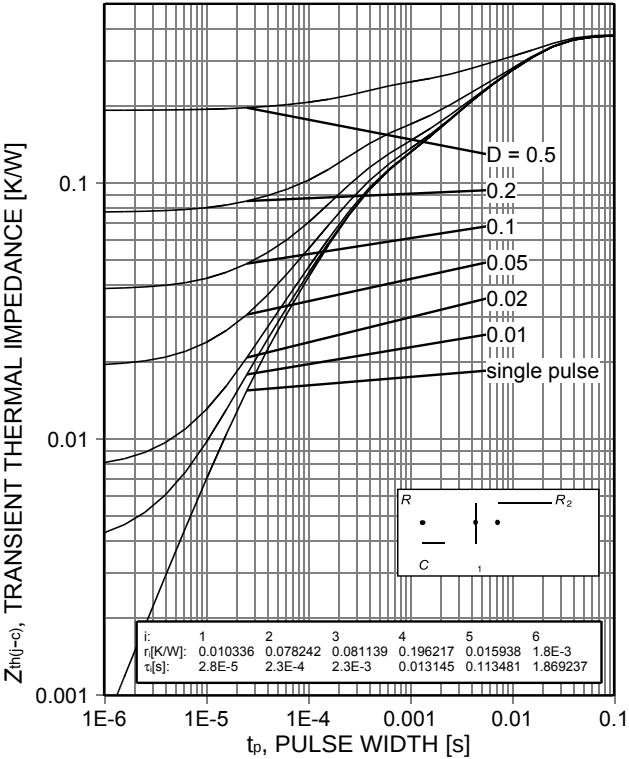
Figure 18. IGBT transient thermal impedance
