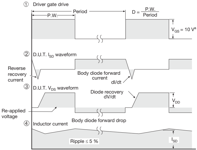
Fig. 18 - For N-Channel
