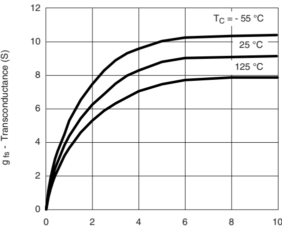
Transconductance
