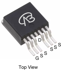
TO-263 7-Lead
