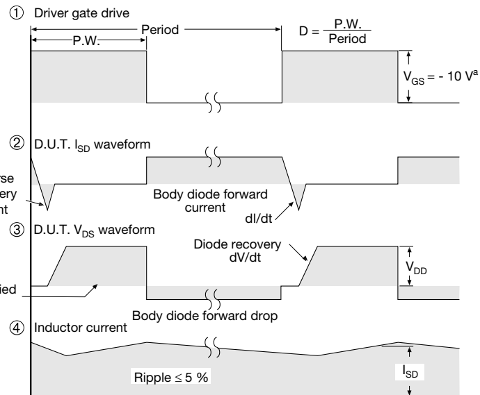
Fig. 14 - For P-Channel
