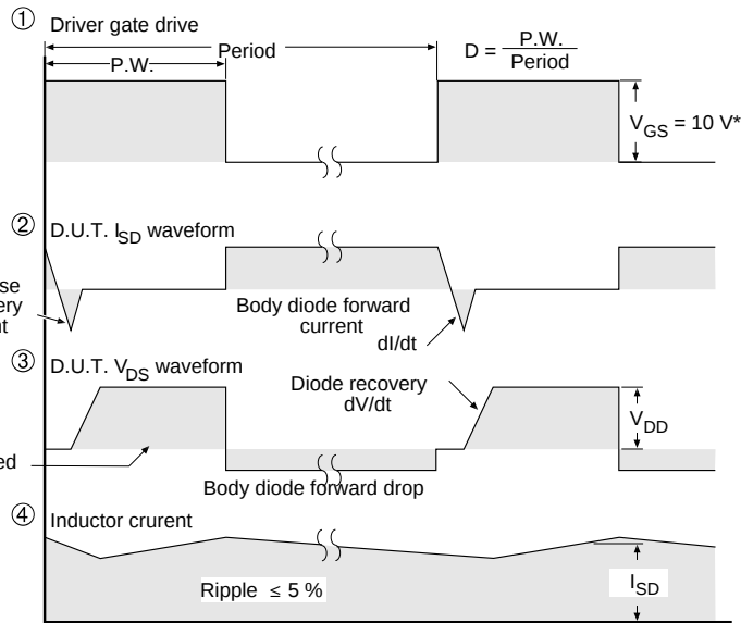
Fig. 14 - For N-Channel
