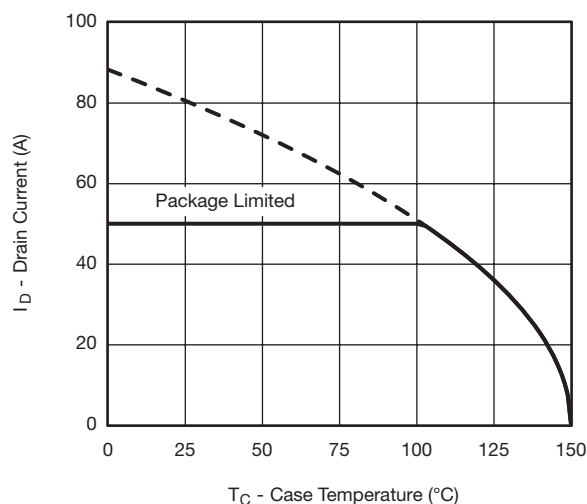
T_C - Case Temperature ( ^\circ\text{C} ) Current Derating
