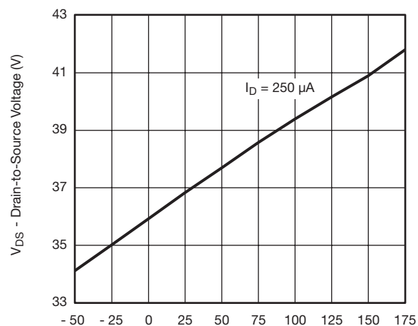
T_J - Temperature ( ^\circ\text{C} ) Drain Source Breakdown vs. Junction Temperature
