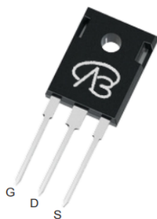
TO-247
