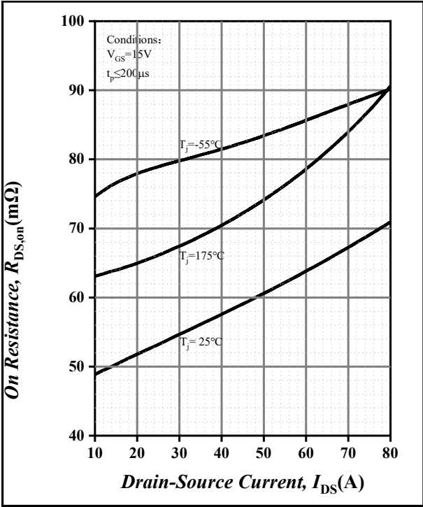
Fig.4 On-Resistance vs. Drain Current For Various Temperatures
