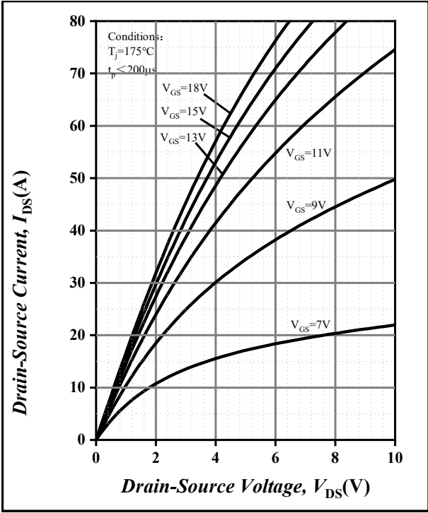
Fig.2 Output characteristics T_j=175^{\circ}\text{C}
