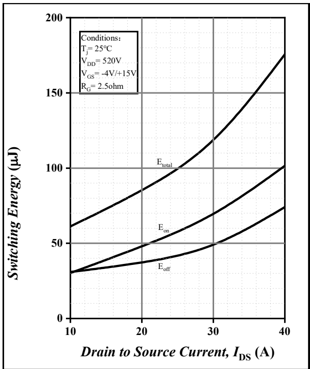
Figure 15. Clamped Inductive Switching Energy vs. Drain Current( V_{DD}=520\text{V} )
