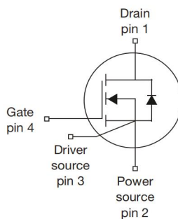
N-Channel MOSFET
