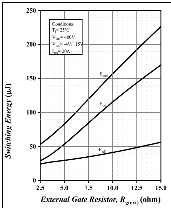
Figure 16. Clamped Inductive Switching Energy vs. R_{g(\text{ext})}
