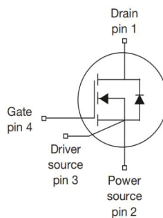
N-Channel MOSFET
