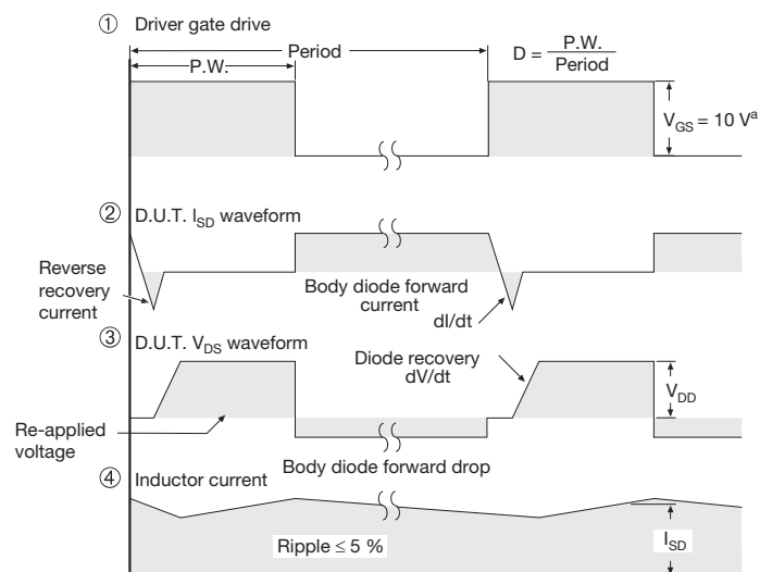
Fig. 18 - For N-Channel
