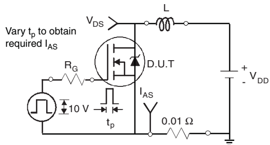
Fig. 14 - Unclamped Inductive Test Circuit
