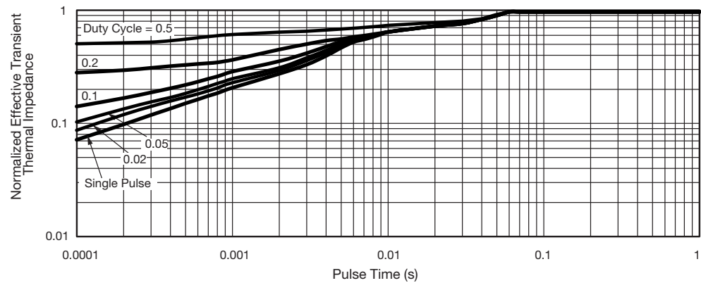
Fig. 11 - Normalized Thermal Transient Impedance, Junction-to-Case
