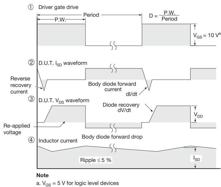
Fig. 18 - For N-Channel
