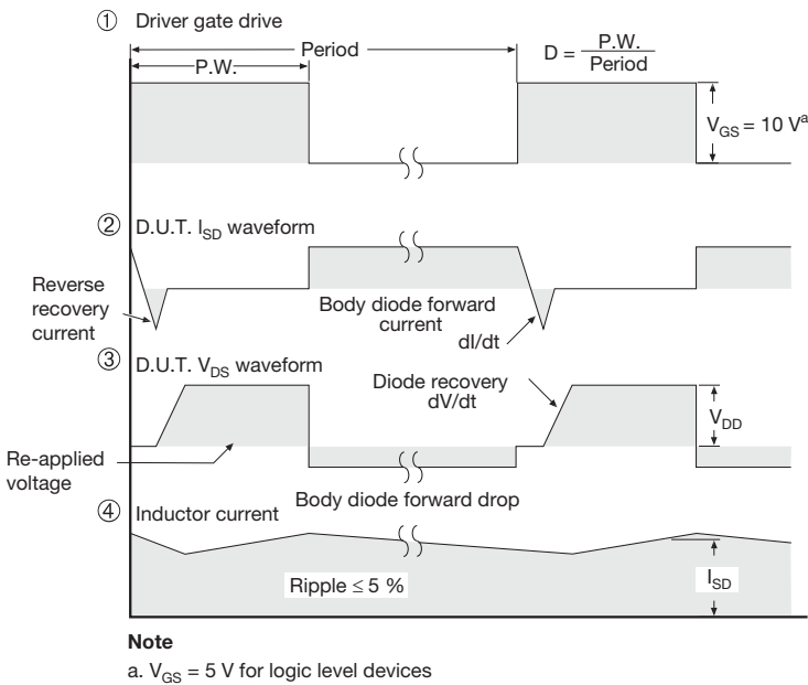
Fig. 18 - For N-Channel
