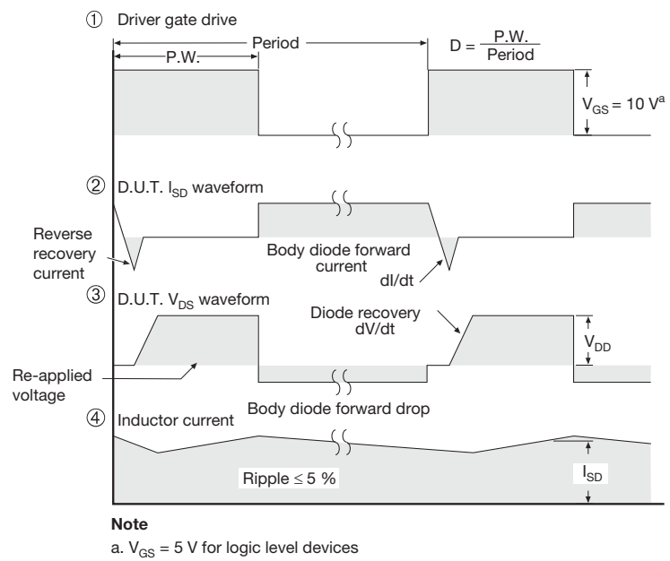
Fig. 18 - For N-Channel
