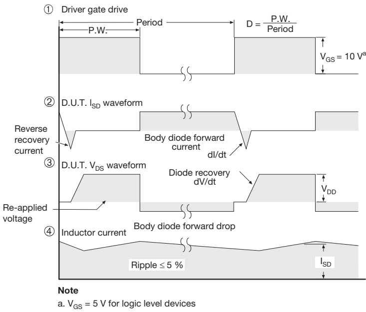
Fig. 18 - For N-Channel
