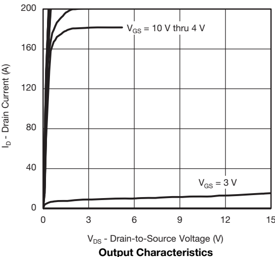
Output Characteristics
