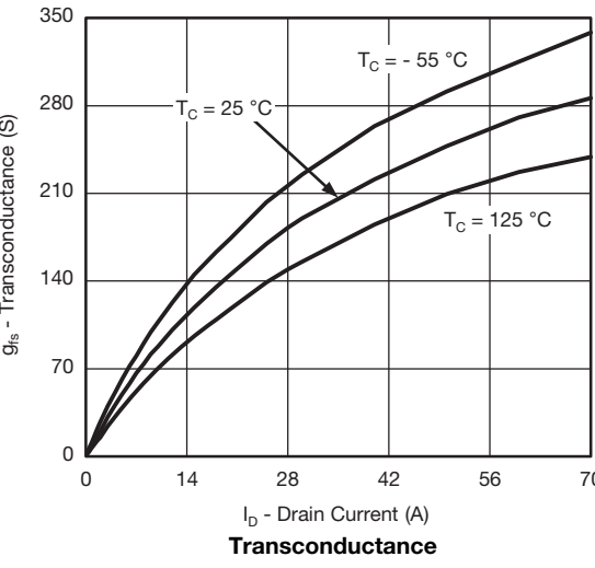
Transconductance
