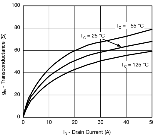
Transconductance
