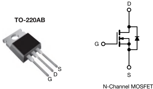
N-Channel MOSFET
