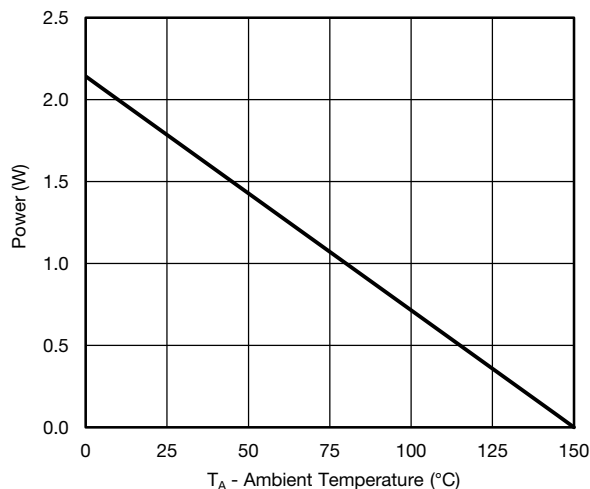
Power, Junction-to-Ambient
