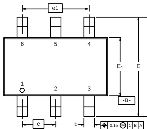
6-LEAD TSOP
