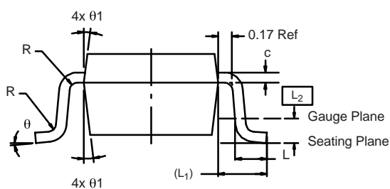
6-LEAD TSOP
