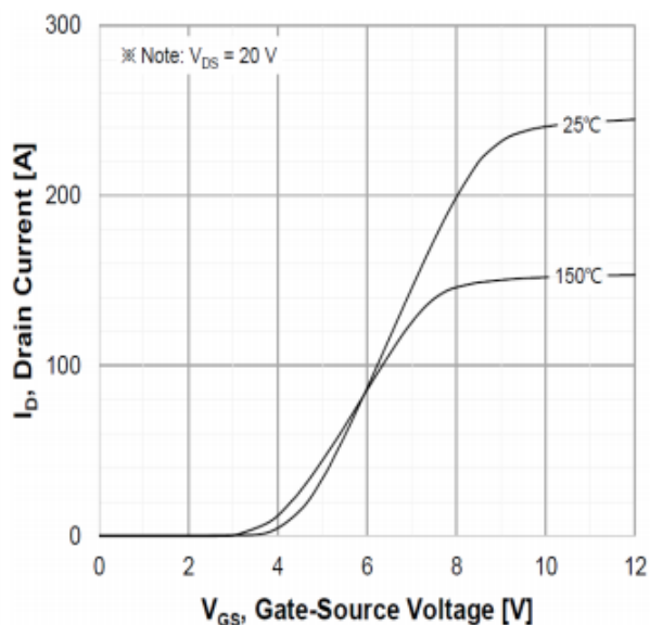
Transfer characteristics
