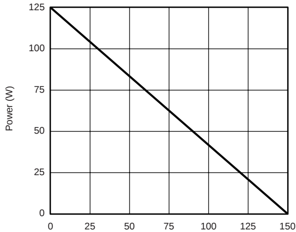
Power, Junction-to-Case
