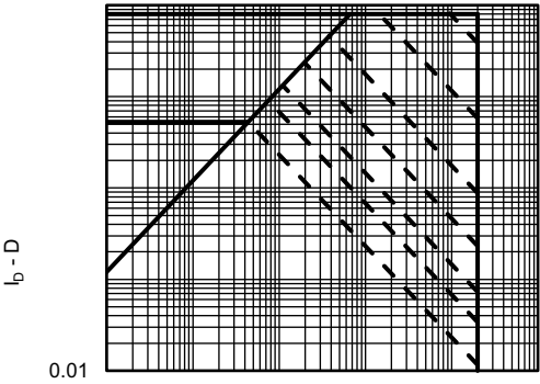
Safe Operating Area, Junction-to-Ambient
