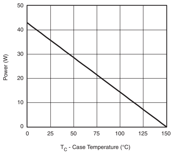
Power, Junction-to-Case
