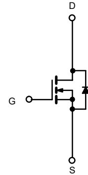
N-Channel MOSFET
