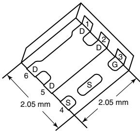
SC-70-6L-Single
